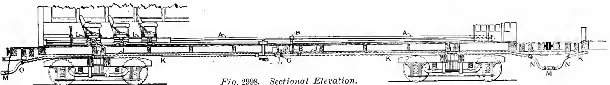
Fig. 2998. Sectional Elevation.
